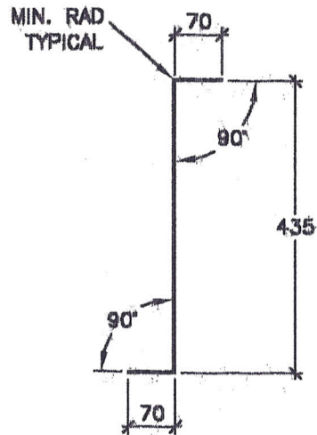
SECTION PROFILE FOR PLATES 1 & 2
