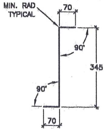
SECTION PROFILE FOR PLATES 1 & 2
